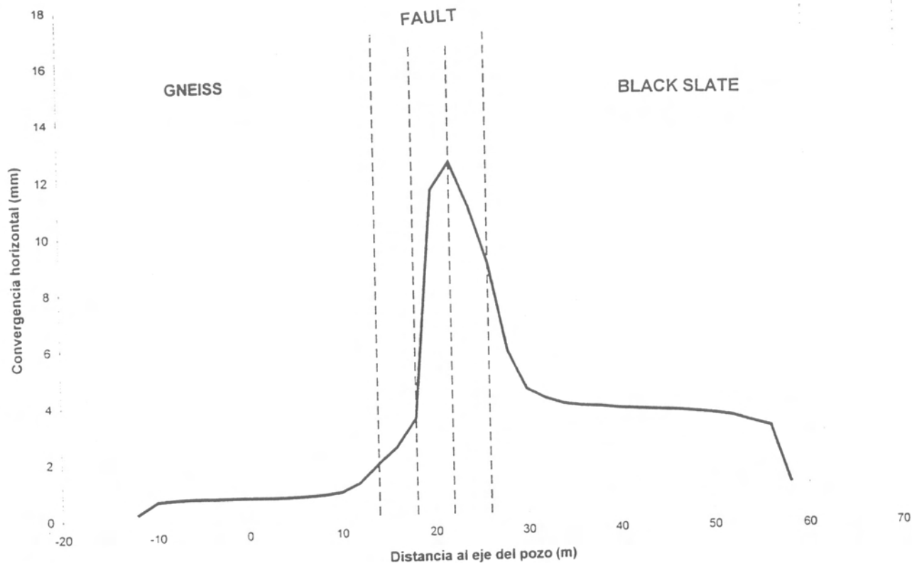
Figure 7.- Convergence profile for K_0 = 1
