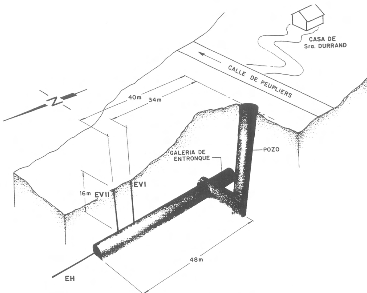
Figure 5.- Instrumentation proposed
