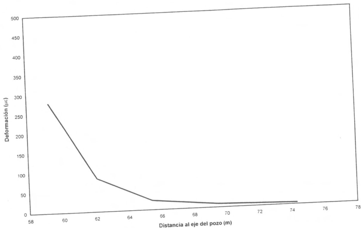
Figure 9.- Strain vs distance for the horizontal extensometers
